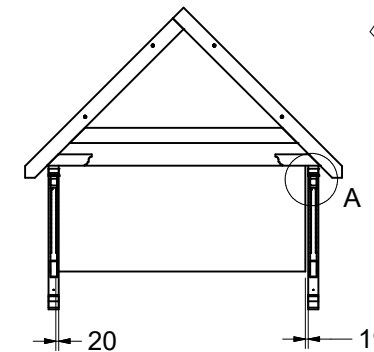
RECOMMENDED CANOPY POSITION WITH DOOR
