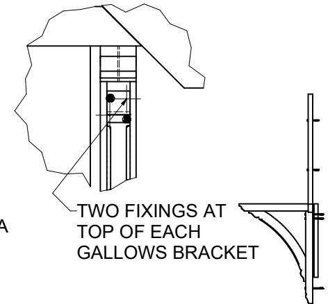
DETAIL VIEW A
